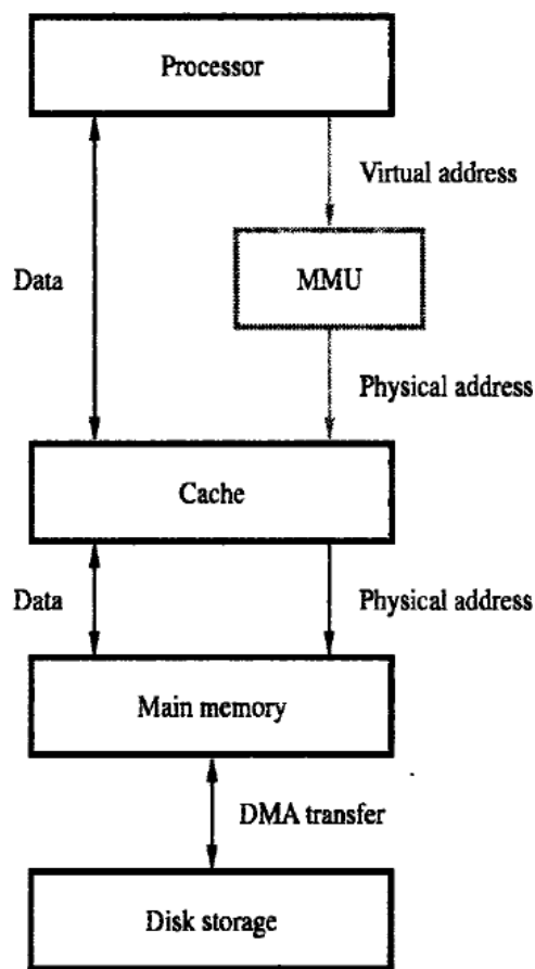
Fig: Virtual Memory Organization
